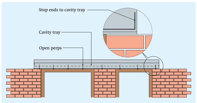
Figure 3 Cavity trays
