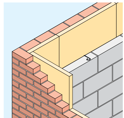
Figure 8 Batts close butted at corners
