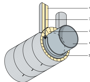
Figure 2 Conlit Ductwork PSM applied to circular duct
