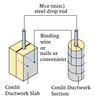
Figure 4 Isometric view of drop rod protection options
